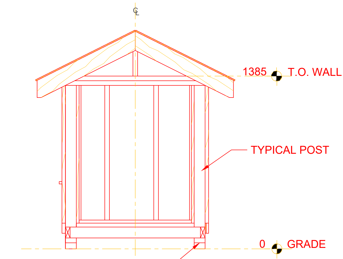
LINE OF BEVEL @ SLEEPER ENDS FRONT-ELEVATION
