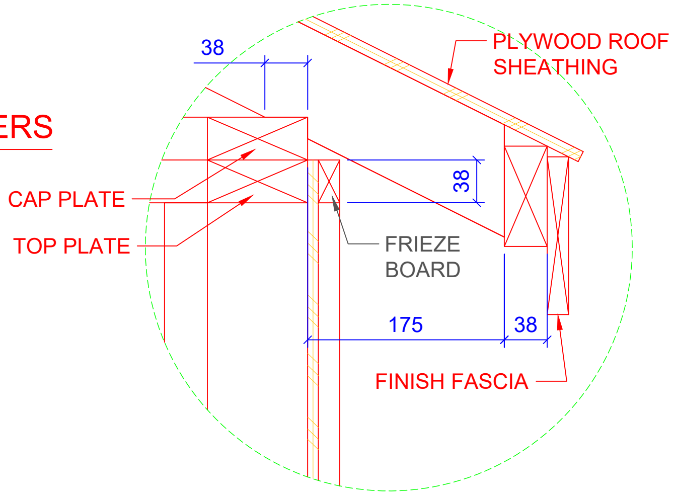
2 TYP. EAVE DETAIL A6
