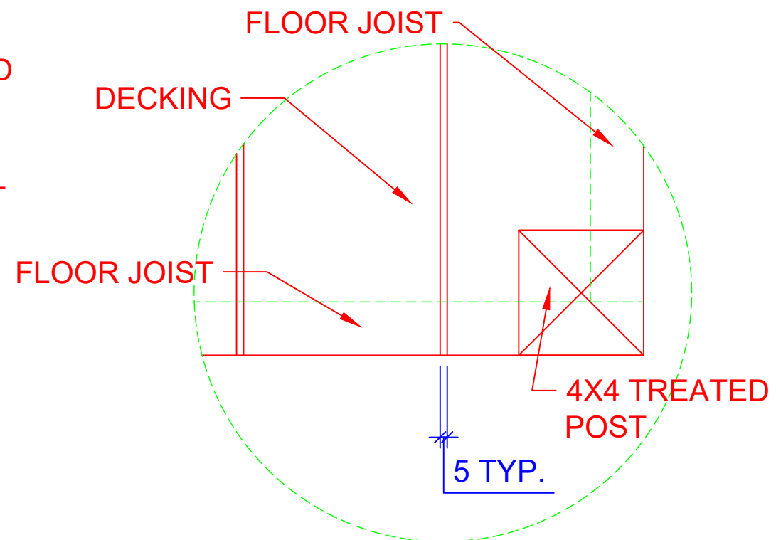
12 DECKING @ FLOOR JOIST A2
