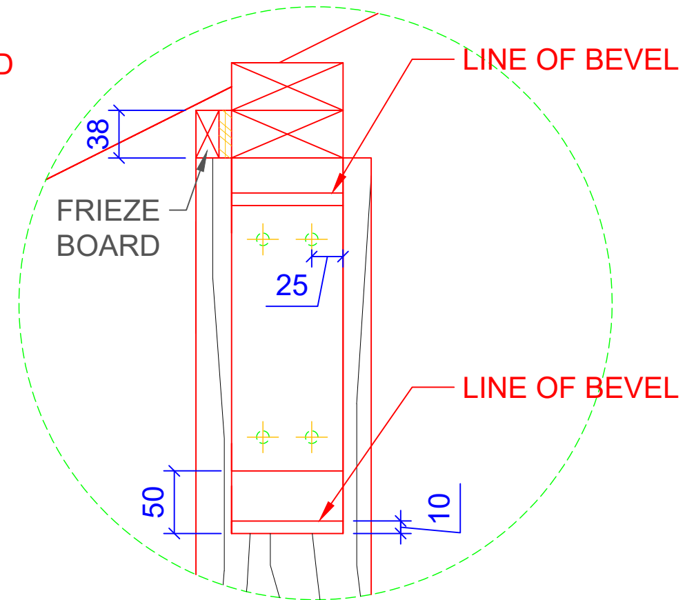
10 BRACE DETAIL-FRONT A6
