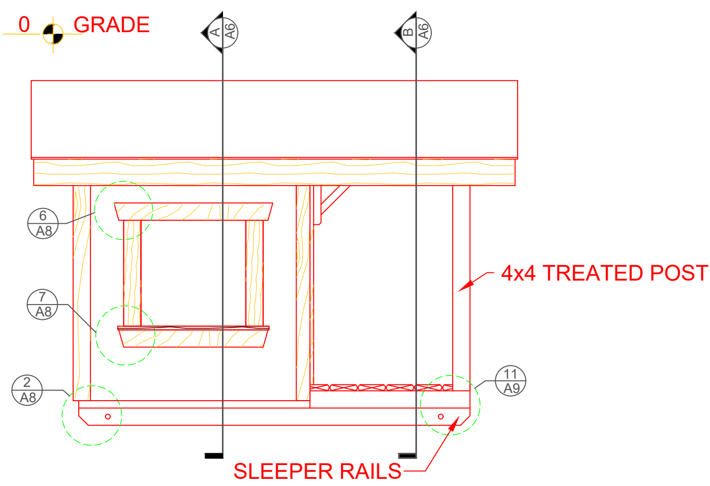
LEFT SIDE-ELEVATION
