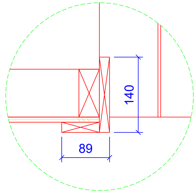
1 FRONT WALL @ CORNERS A2
