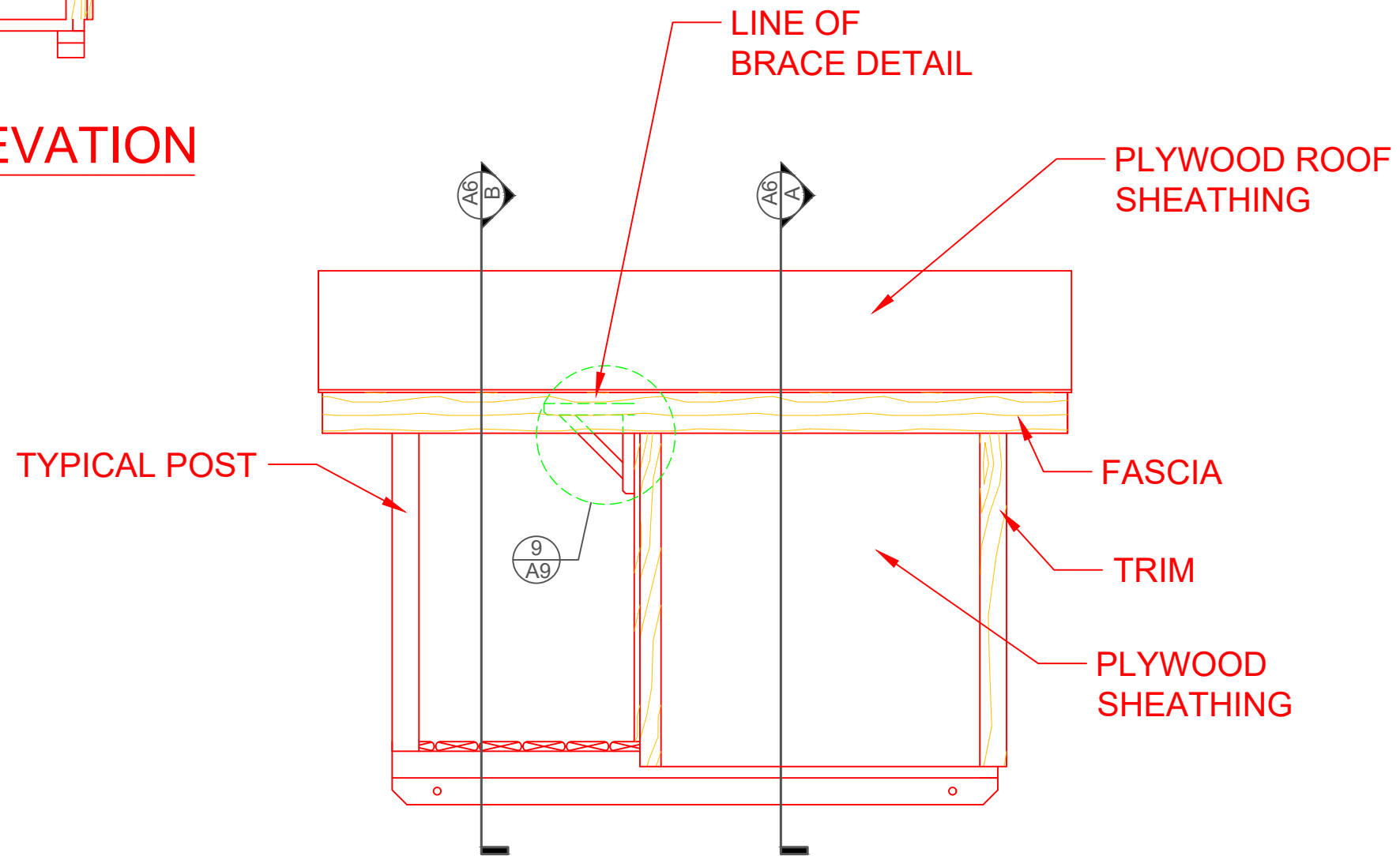
RIGHT SIDE-ELEVATION
