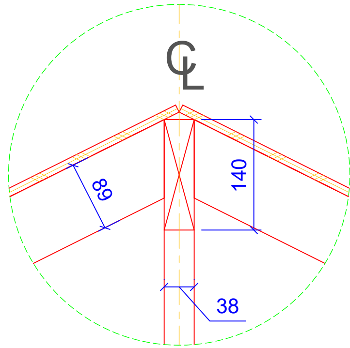
4 RIDGE DETAIL A6
