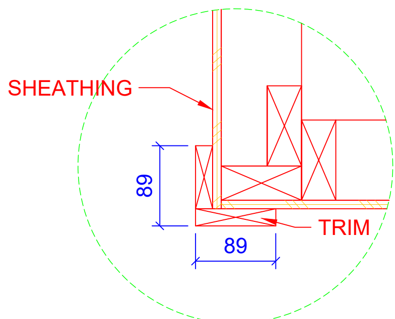
3 BACK WALL @ CORNERS A2
