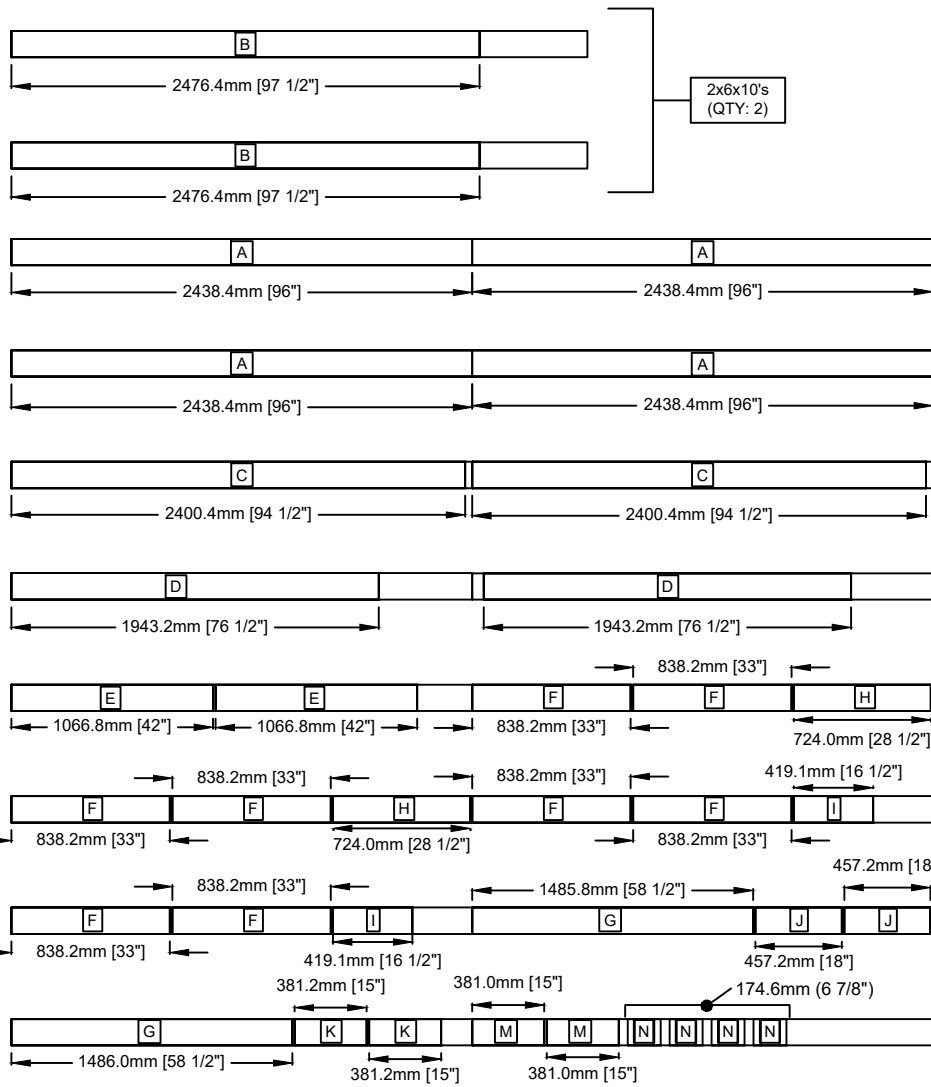
1 2x6" LUMBER DIMENSIONS SCALE = 1:40
