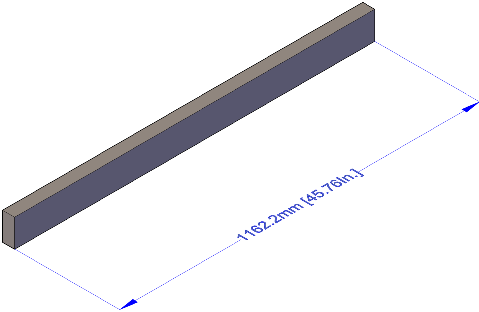
2x4 DIVIDER WALLS (QUANTITY = 6) - LENGTH = 45.76 In.
