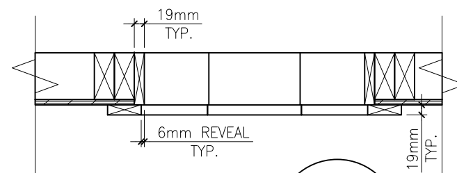
SECTION F-F TYPICAL BRACE SCALE 1:10
