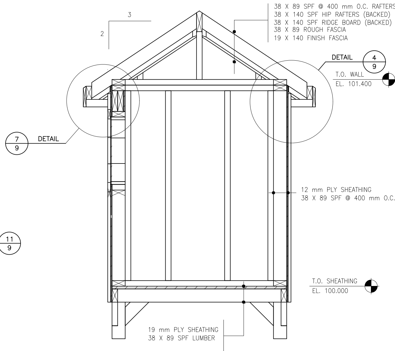
SECTION B-B SCALE 1:15 2
