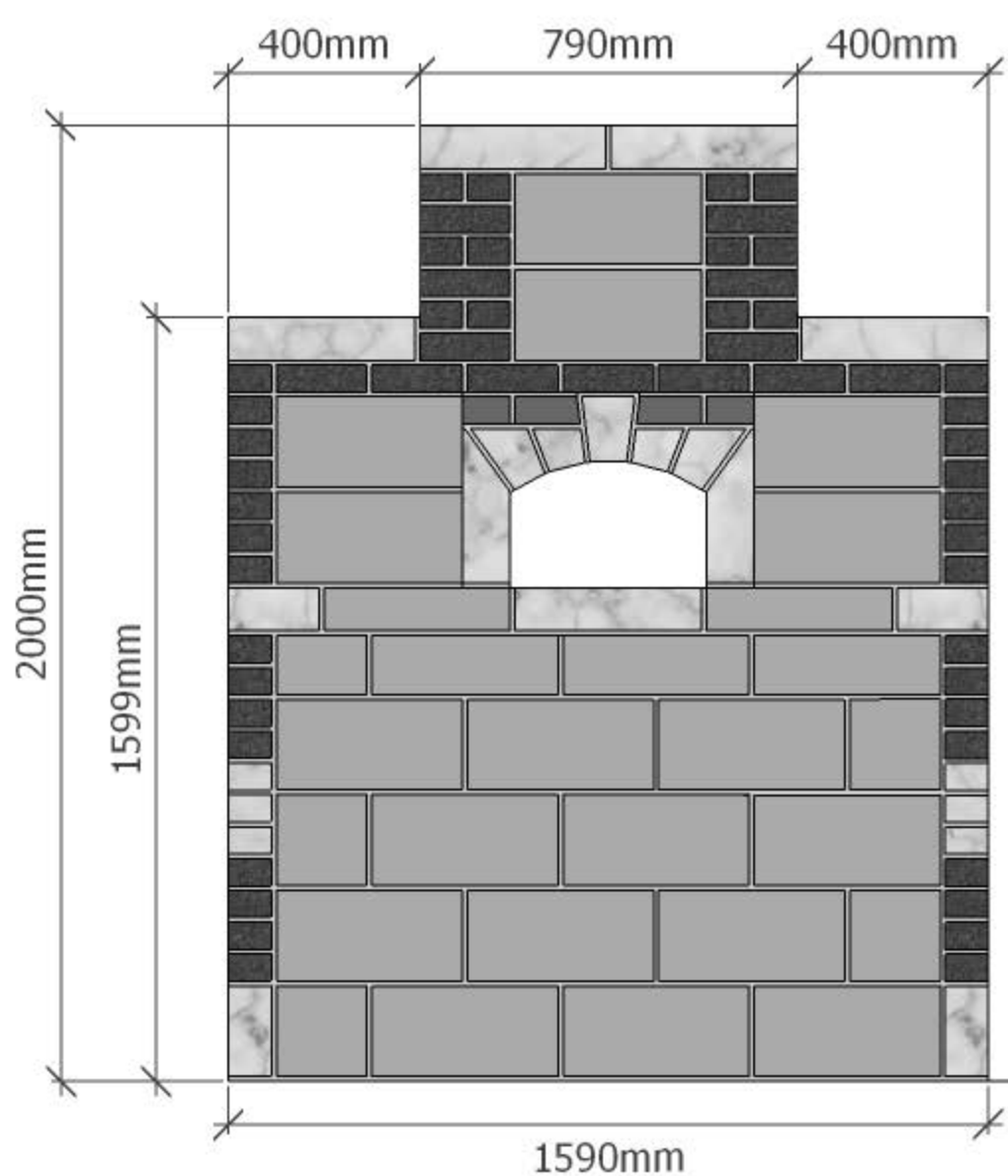
COMPLETE REAR ELEVATION
