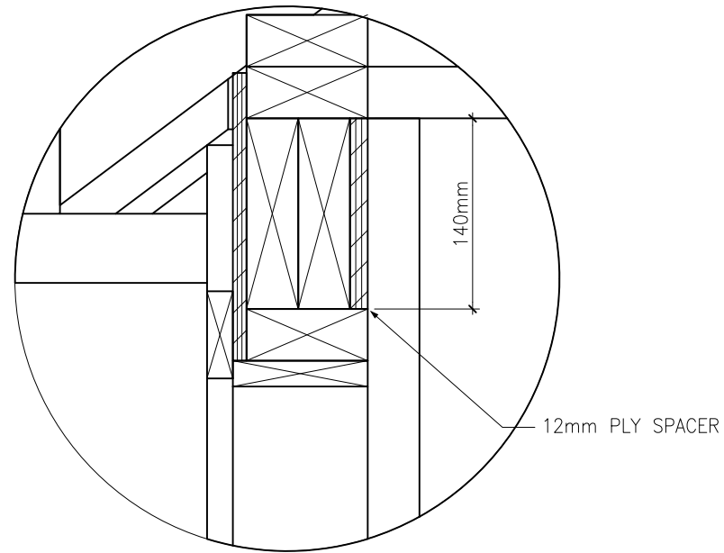
DETAIL 3 LINTEL DETAIL 7
