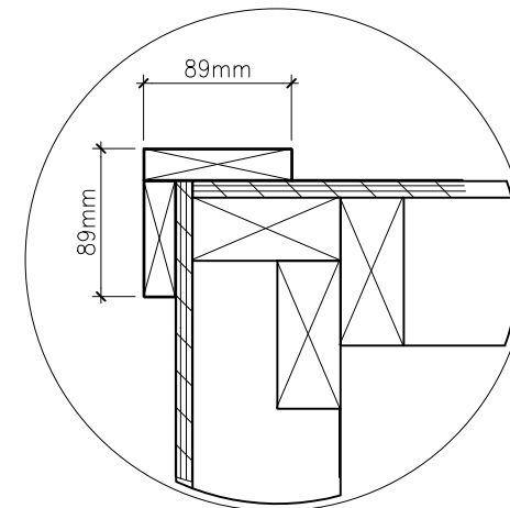
DETAIL 1 REAR WALL TRIM DETAIL TYPICAL 2
