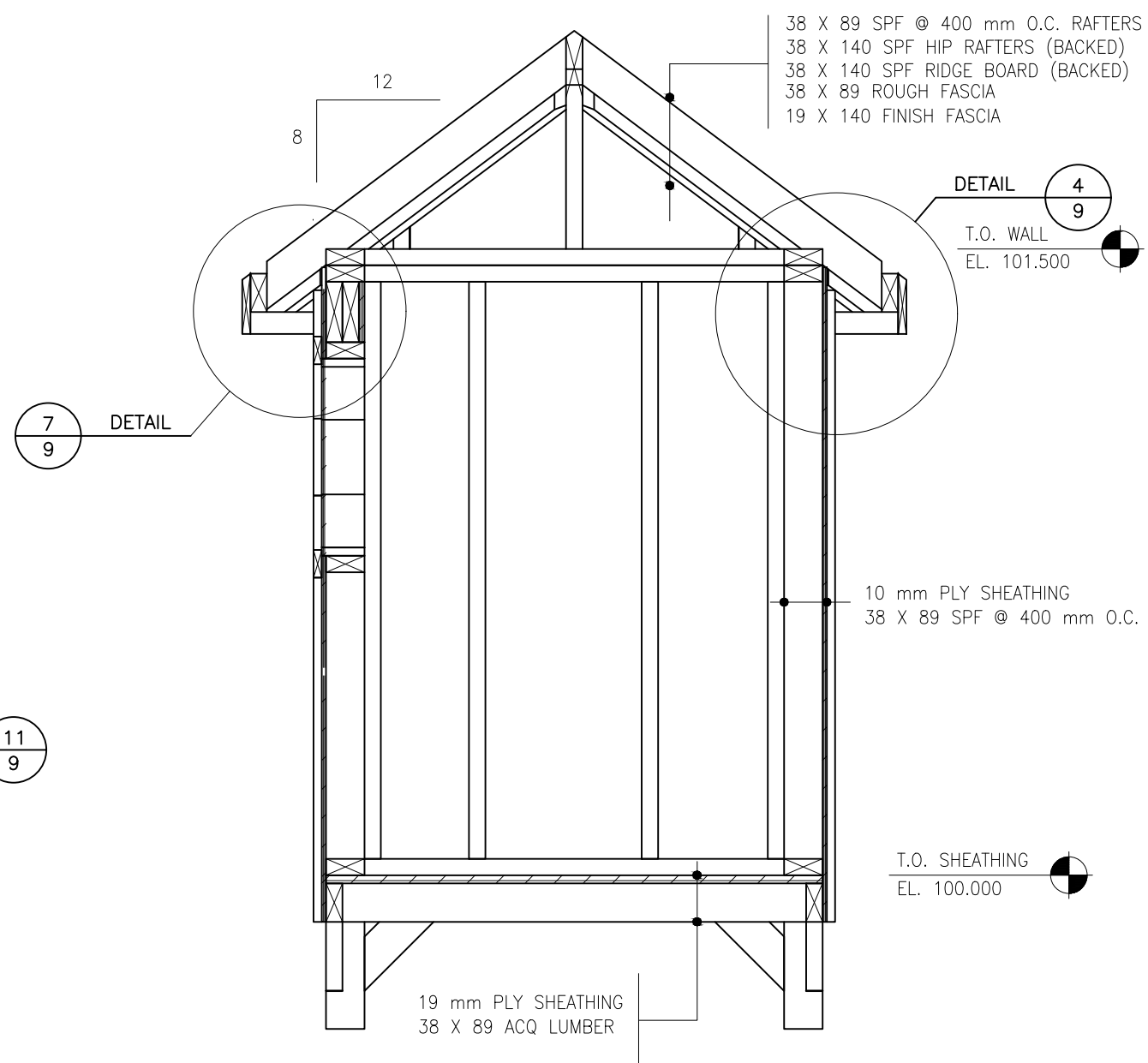
SECTION B-B SCALE 1:15
