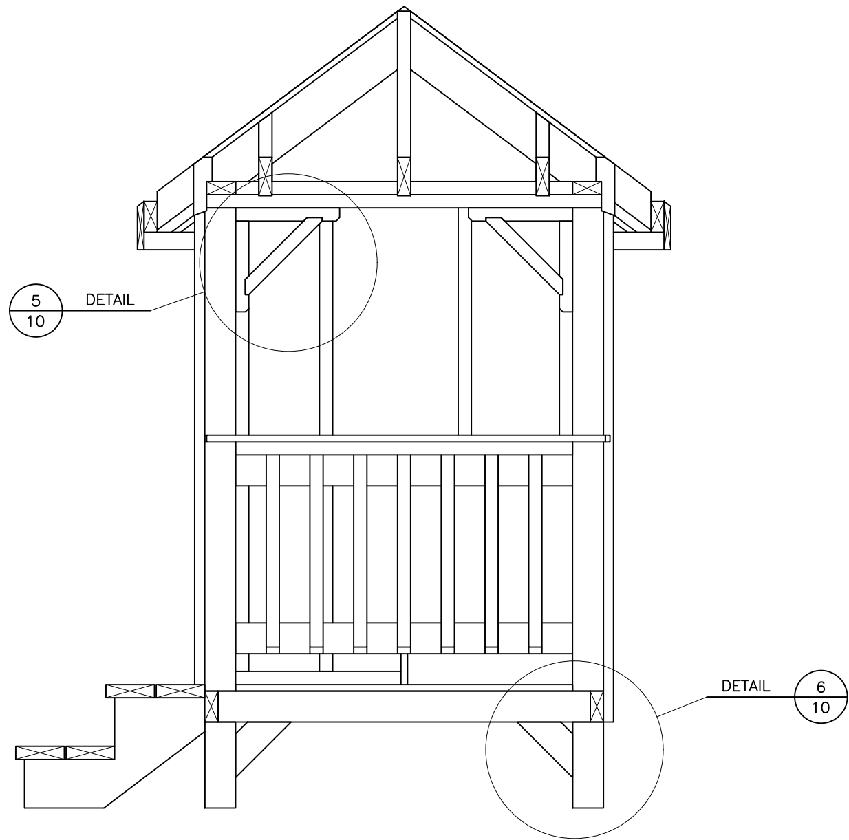
SECTION C-C SCALE 1:15
