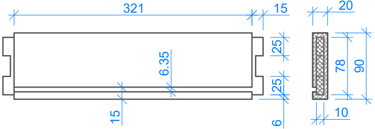
SIDE RAILS Scale 1:5
