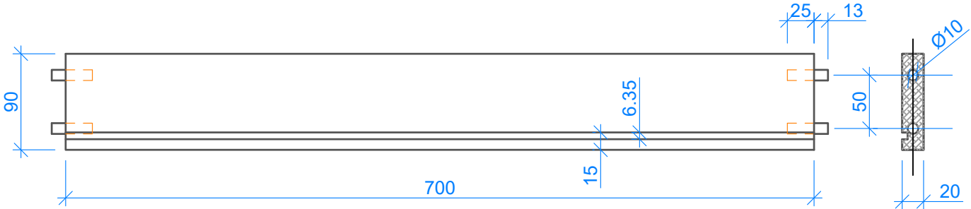
BACK RAIL Scale 1:5
