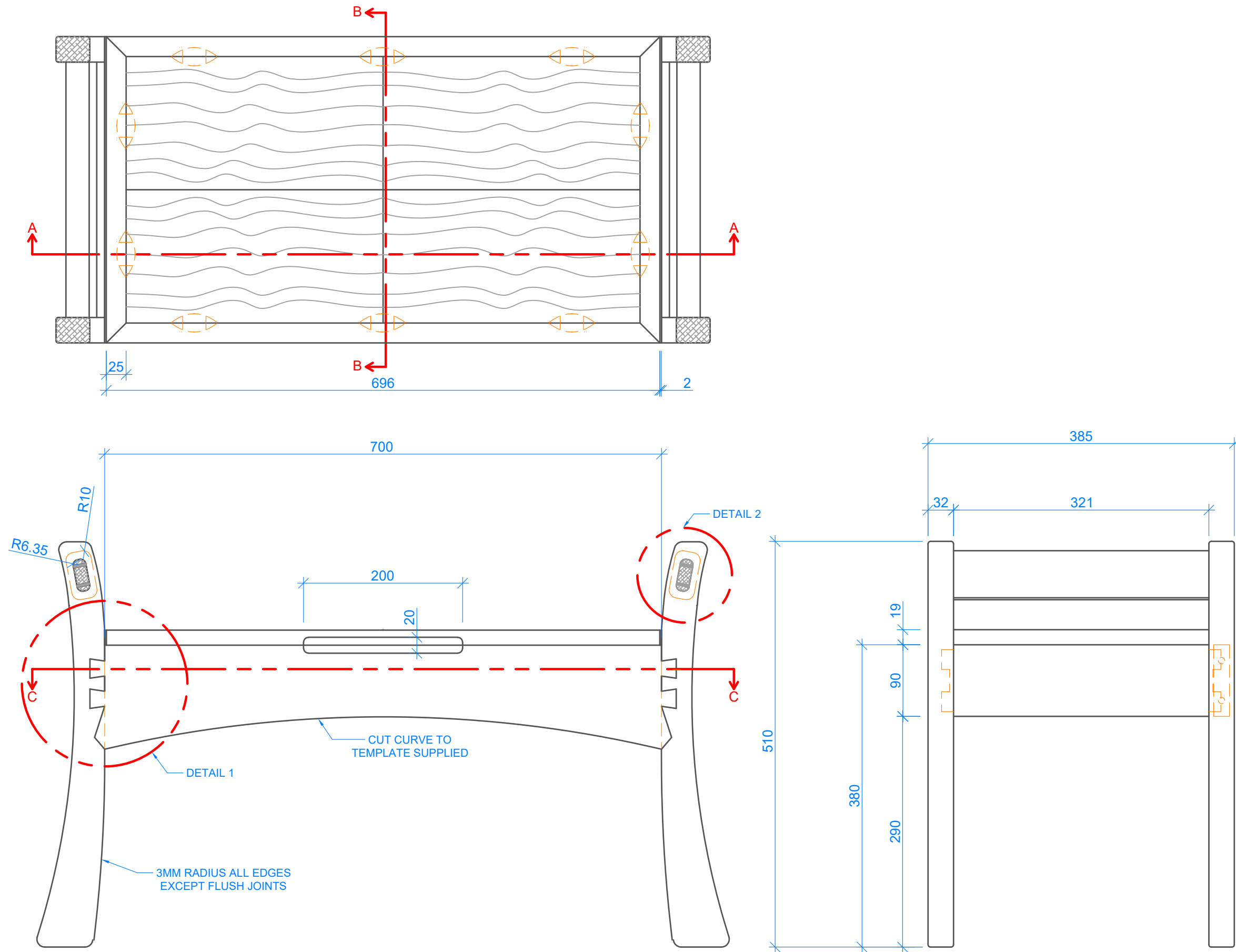
Top, Front and Right Side Views Scale 1 : 5
