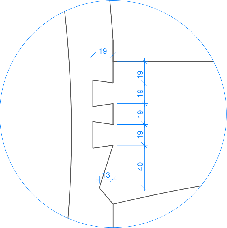
DOVETAIL HALF LAP LAYOUT Scale 1:2
