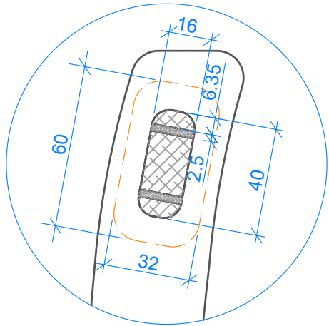
TOP RAIL OF END FRAME JOINERY DETAILS Scale 1:2
