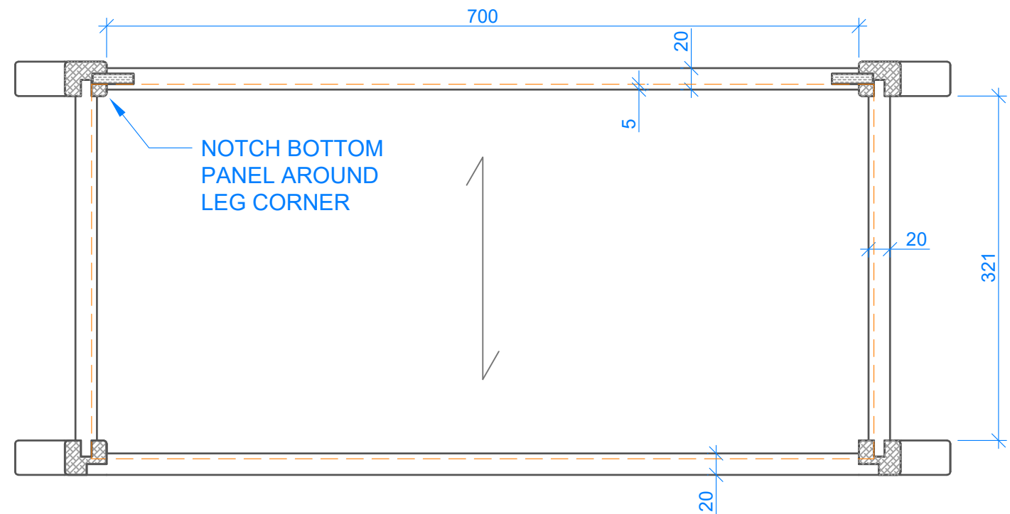
SECTION C-C
