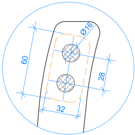
TOP RAIL OF END FRAME JOINERY DETAILS SCAE 1:2
