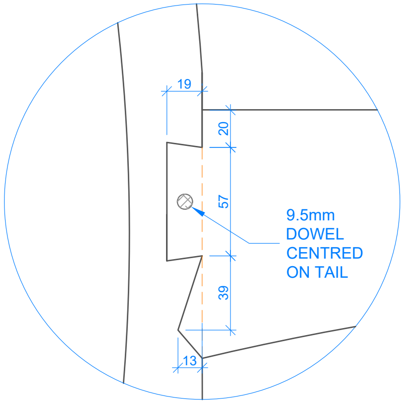
DOVETAIL HALF LAP LAYOUT SCALE 1:2
